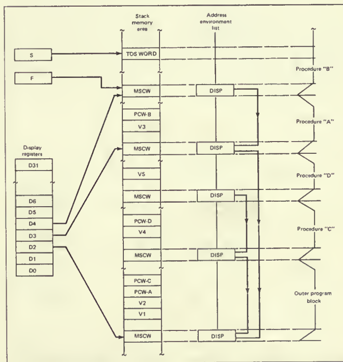
Fig. 5. Display registers indicating current addressing environment.
