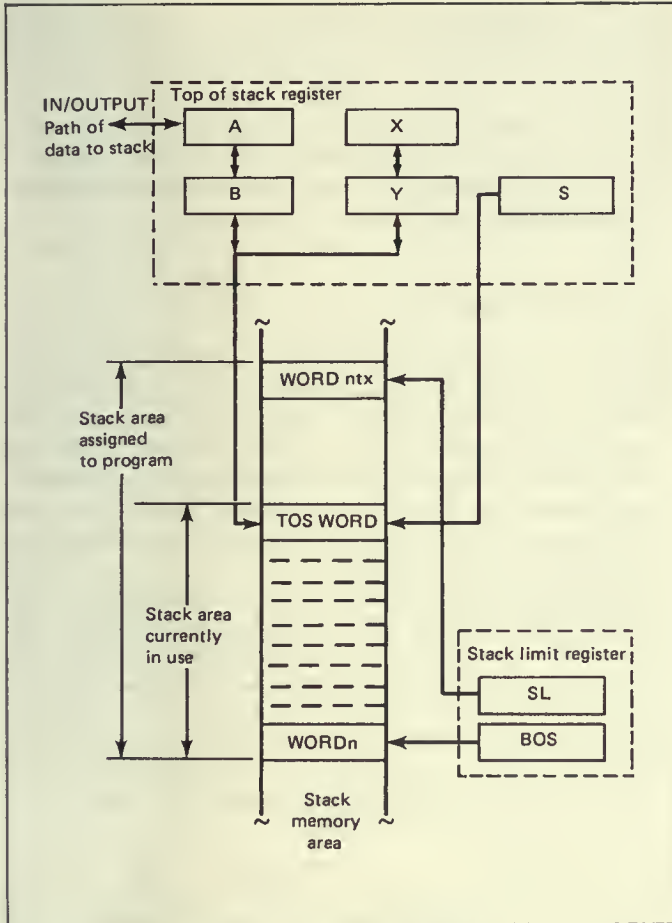
Fig. 2. Top of stack and stack bounds registers.
