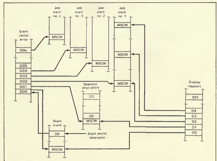
Fig. 7. Multiple linked stacks.
