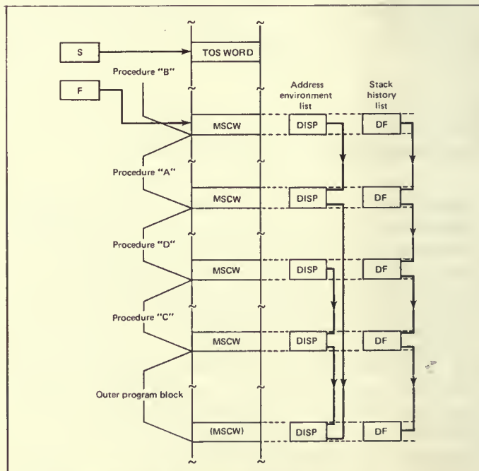
Fig. 3. Stack history and addressing environment list.
