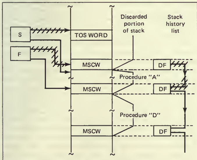
Fig. 4. Stack cut-back operation on procedure exit.
