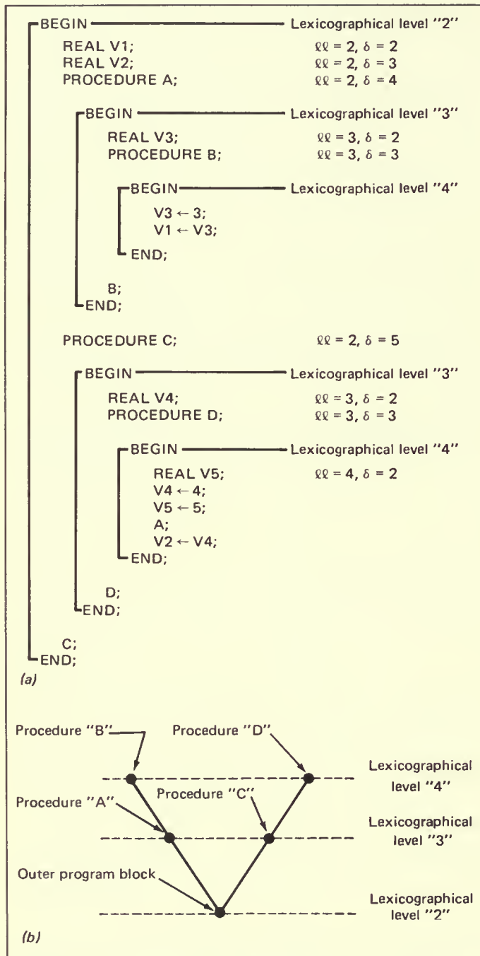
Fig. 6. (a) ALGOL program with lexicographical structure indicated. (b) Addressing environment tree of ALGOL program in (a).
