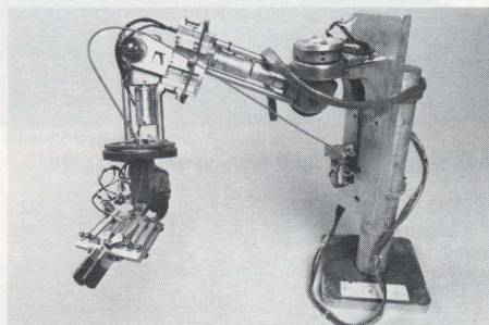
Photo Dan McCoy/Rainbow Rancho Arm, on loan from Stanford University, Stanford, Calif.
